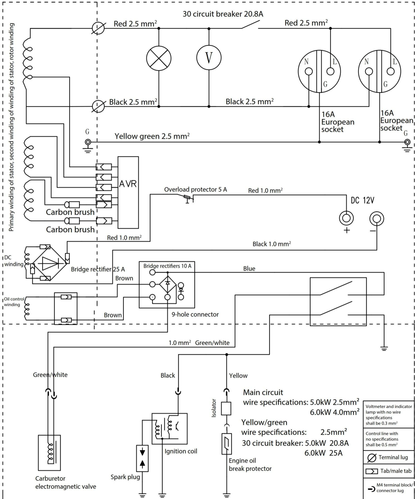
Electrical Schematic Diagram
